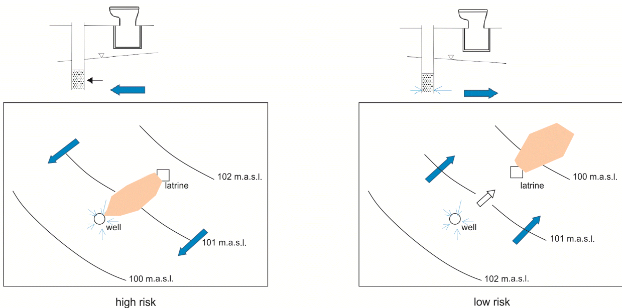
Figure 5: Example: These map examples show the contours for groundwater head above an agreed standard – here in meter above sea level (m.a.s.l.). The blue arrows show the direction of groundwater flow (from high to low head). To decrease the risk to the well, the sanitation system should be located down-gradient of the groundwater supply system (right figure). This should be proven by repeated measurements at several wells during several years.
