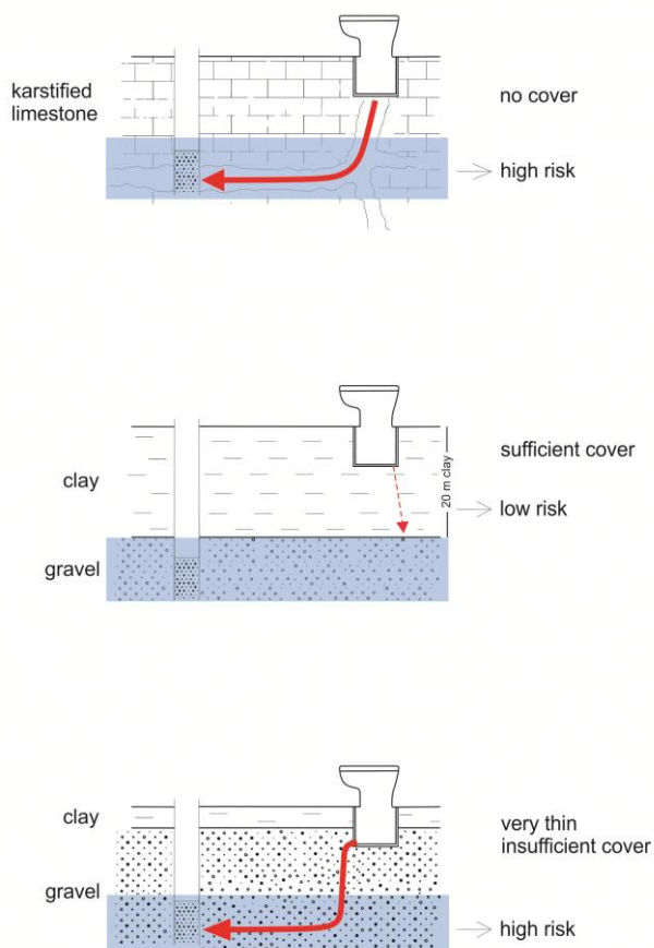
Figure 6: (a) high risk setting due to lack of cover sediments (b): low risk setting due to thick clay sequence acting as barrier (c) high risk setting due to insufficient depth of cover sediments (e.g. clay).
