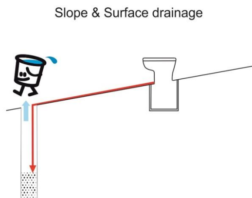
Figure 7: Example for strong increase in risk: septic tank 20 m uphill of the water supply well which does not have a properly constructed sanitary sealing /defect headworks.
