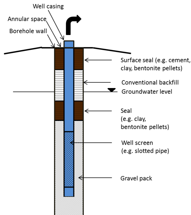
Figure 3: Example for placement of sealings.
