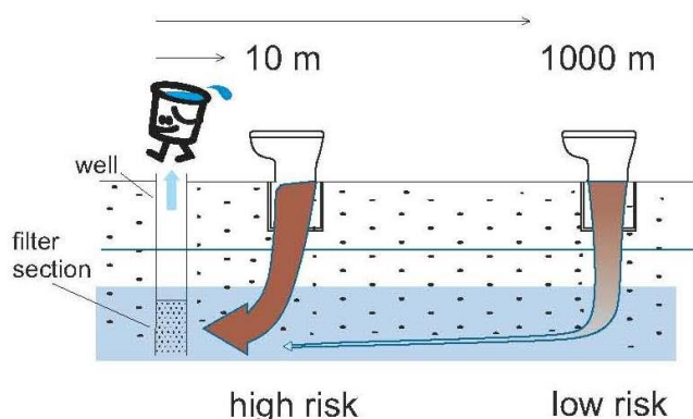
Figure 1: Example for high and low risk due to different horizontal separation distances.
