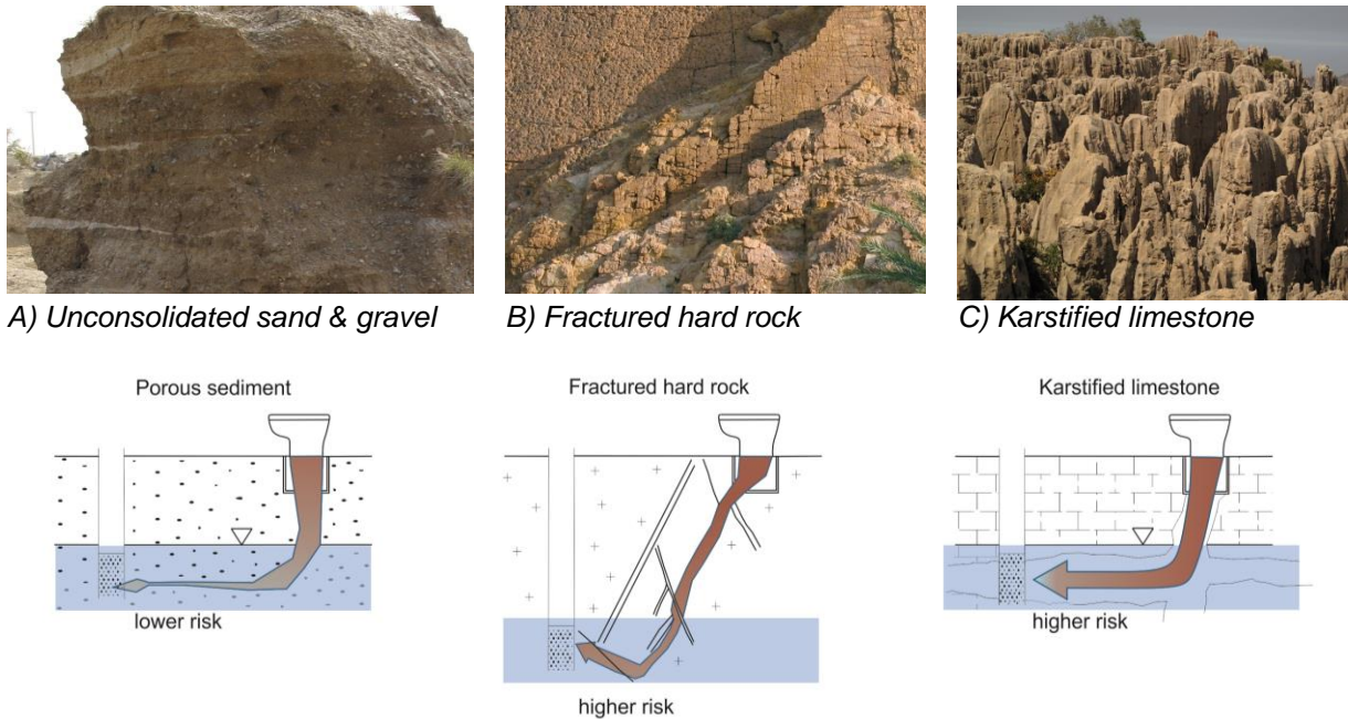
Figure 4: Different aquifer types leading to different risk levels. A) Example for lower risk: unconsolidated sand and gravel aquifer. B) Example for higher risk: fractured hard rock, C) Example for highest risk: karstified limestone. (Photographs by Kai Hahne, BGR)
