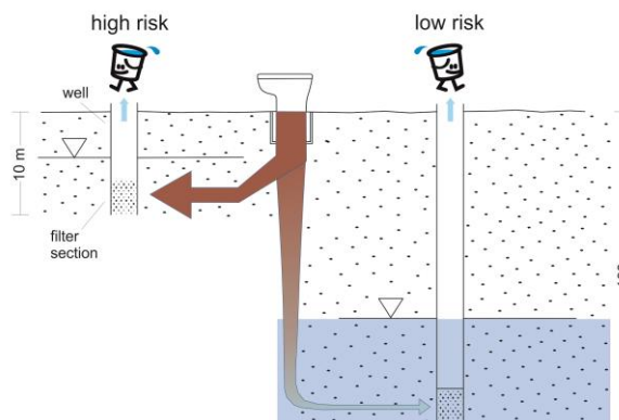
Figure 2: Lower risk with greater depth: A) Example for significant increase in risk: Dugwell with less than 10 m depth in permeable aquifers. B) Example for significant decrease in risk: Well with screened depths of more than 100 m below surface and appropriate sealing of the annular space (see also Figure 7).
