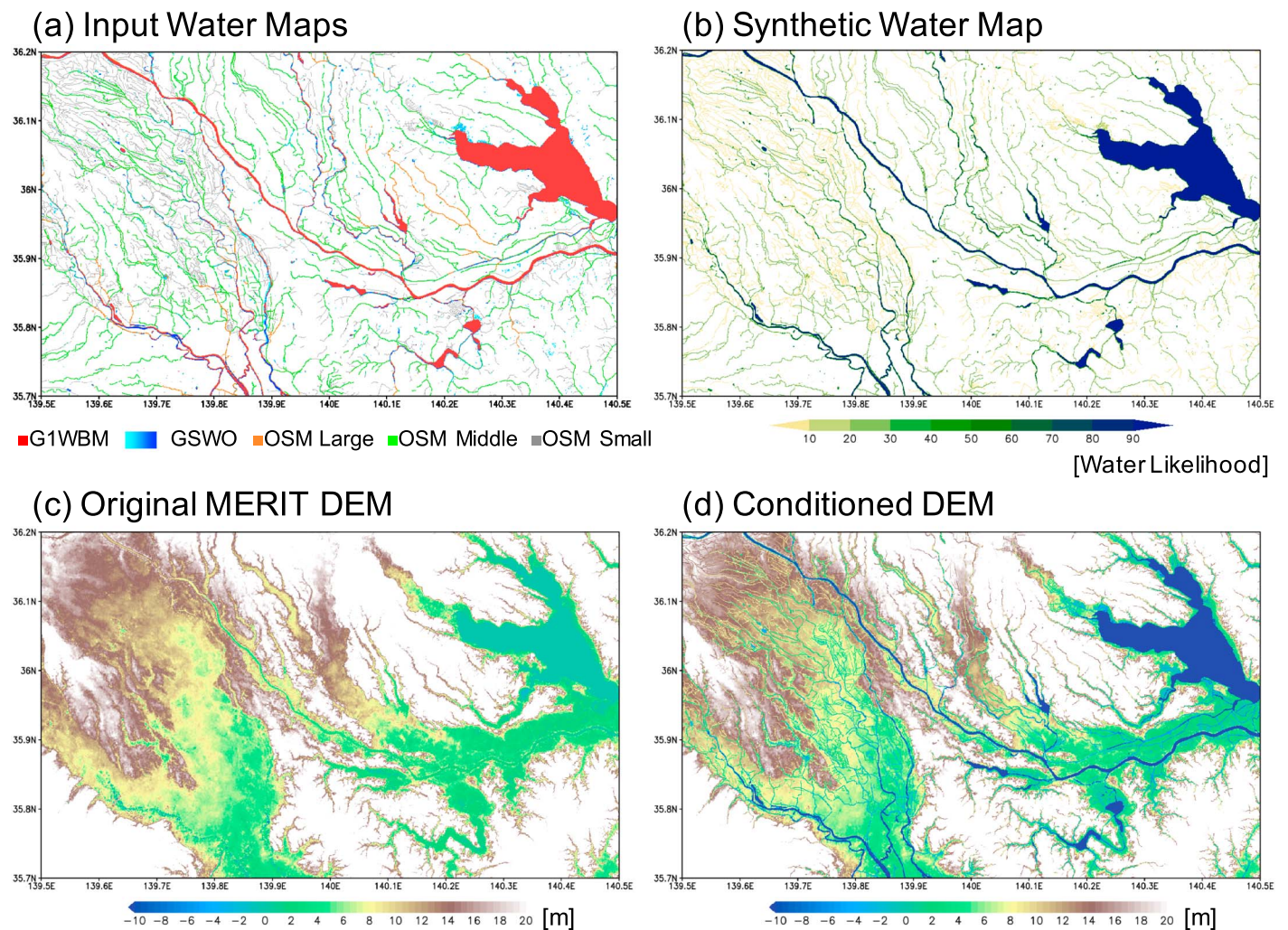
Figure 2. Elevation conditioning for initial flow direction calculation for the Tone River in Japan. (a) Input water maps. (b) Synthetic water layer data. (c) Original MERIT DEM elevation. (d) Conditioned DEM elevation. G1WBM = Global 1-s Water Body Map; GSWO = Global Surface Water Occurrence; MERIT DEM = Multi-Error-Removed Improved-Terrain digital elevation model.
