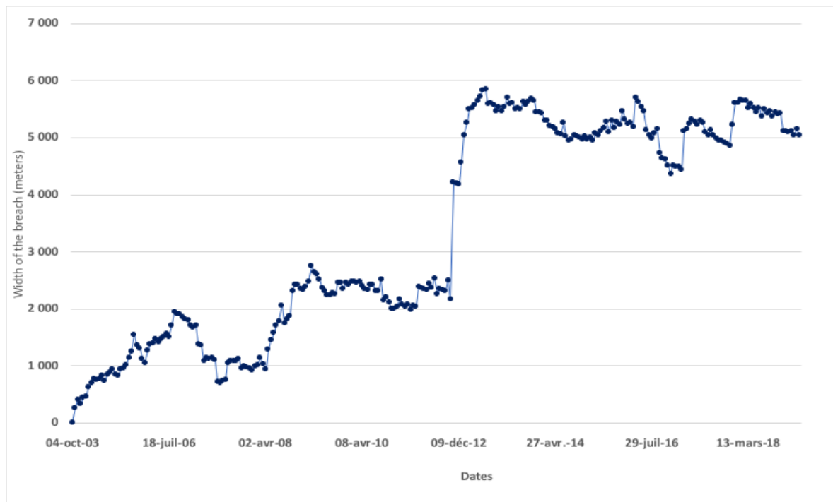
Figure 41: Reconstruction of the widths of the breach from its opening to October 2018 (data calculated from LANDSAT satellite imagery)
