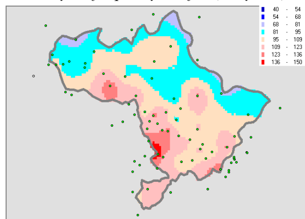
Perennial frequency rainfall (1/20 years)
