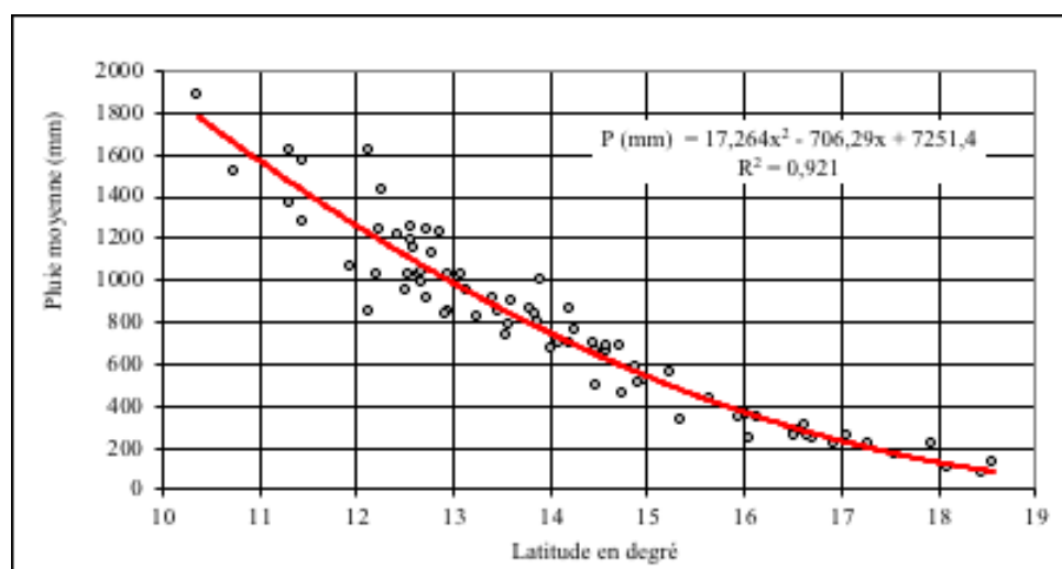
Figure 13: Correlation between precipitation and latitude (in degrees)
