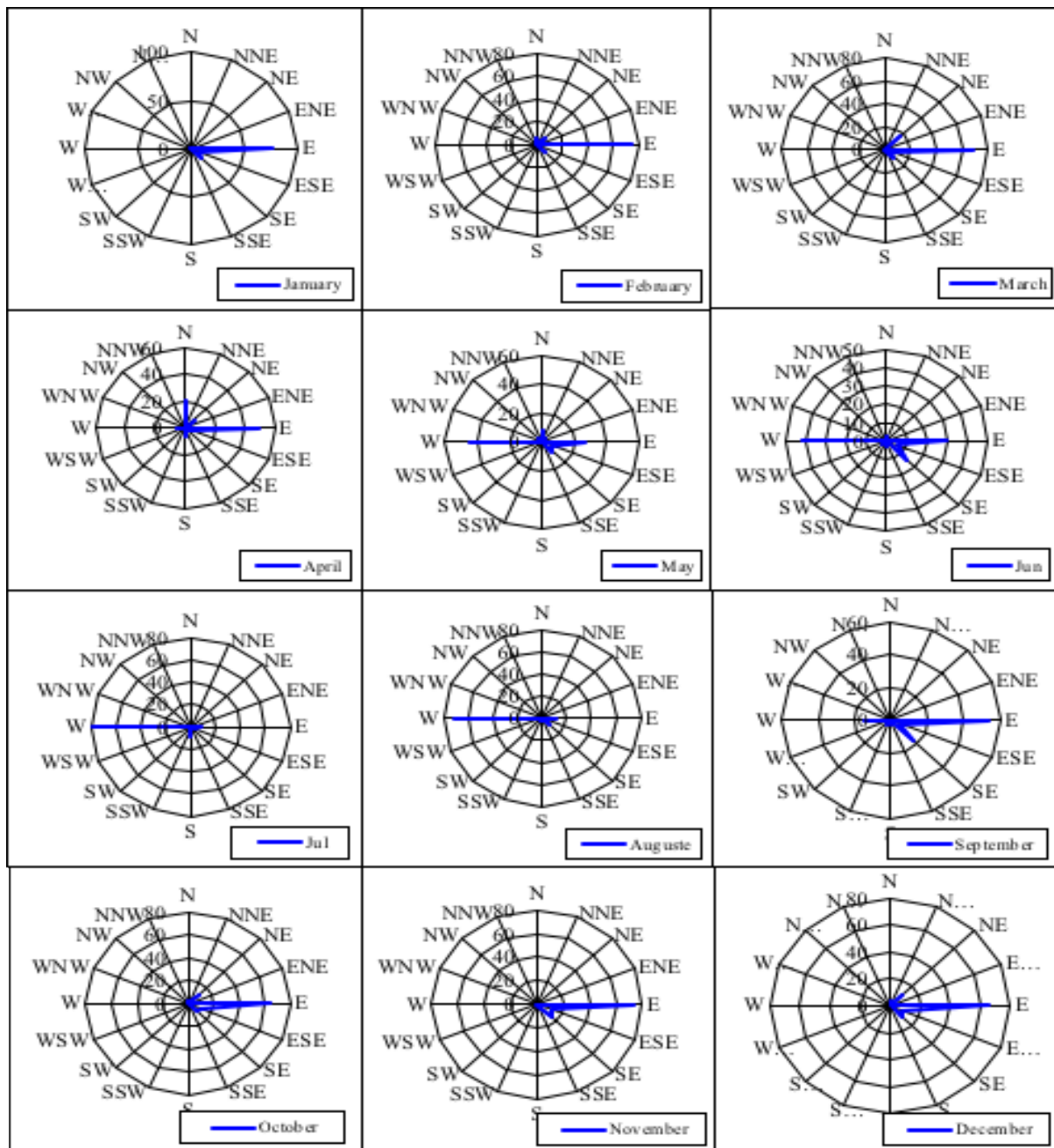
Figure 9: Wind rose at Labe Station
