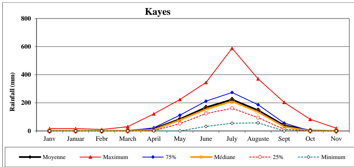
Figure 19 : Monthly rainfall profiles of Mamou, Siguiri, Kéniéba and Kayes
