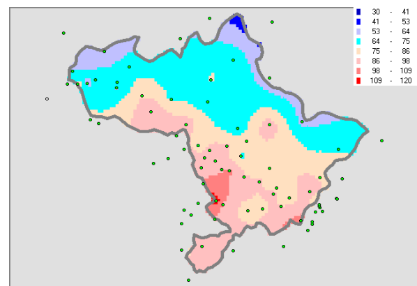
Five-year frequency rainfall (1/5 years)
