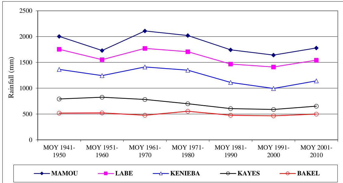
Figure 18 : Variations in ten-year average rainfall at a few stations in the basin
