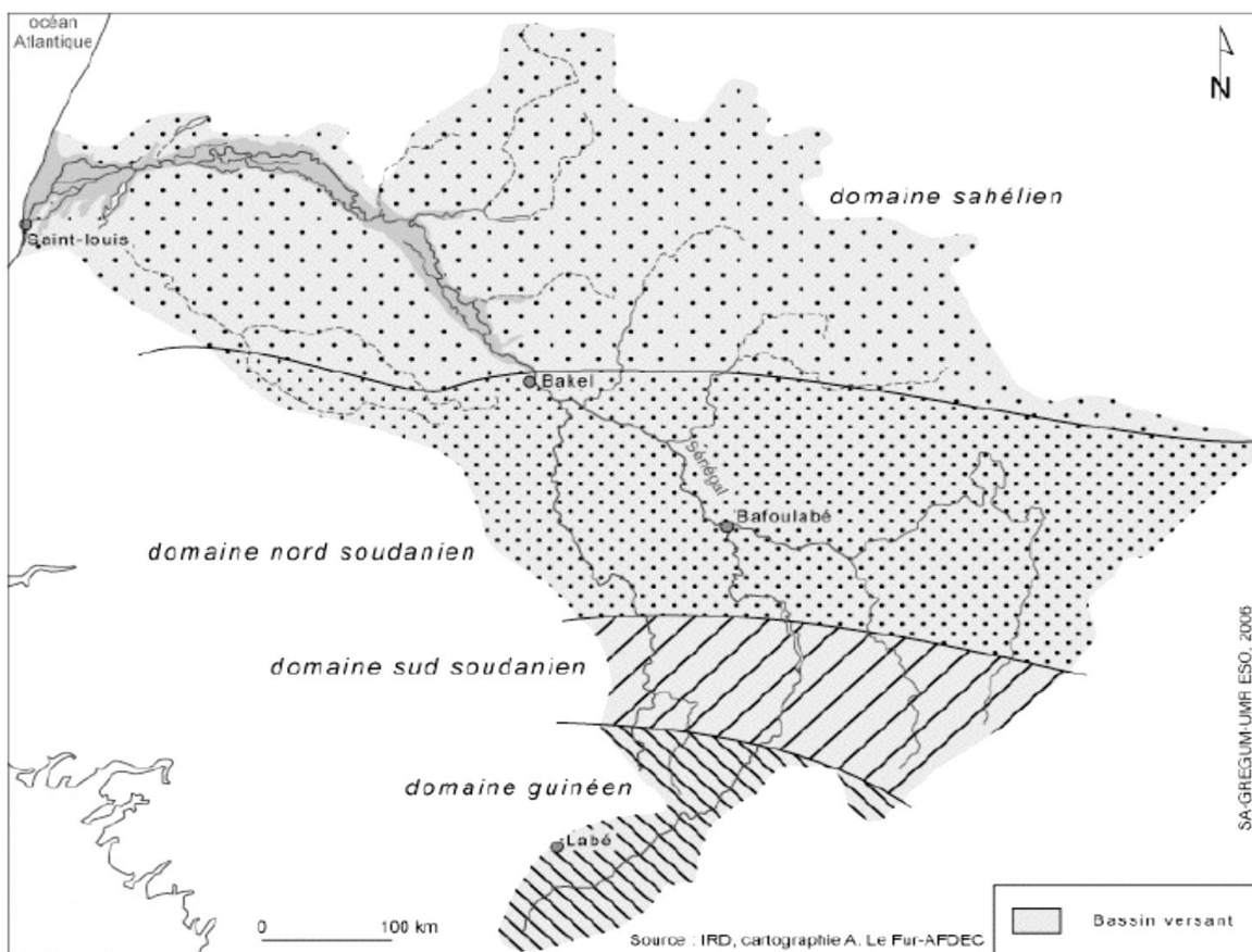
Figure 4: Climate domains of the Senegal River Basin (modified by SALL (2006) from SOW (1984))
