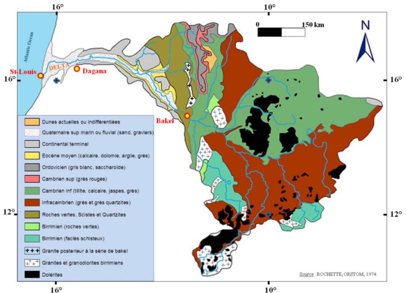
Figure 2: Geological Map of Senegal River Basin
