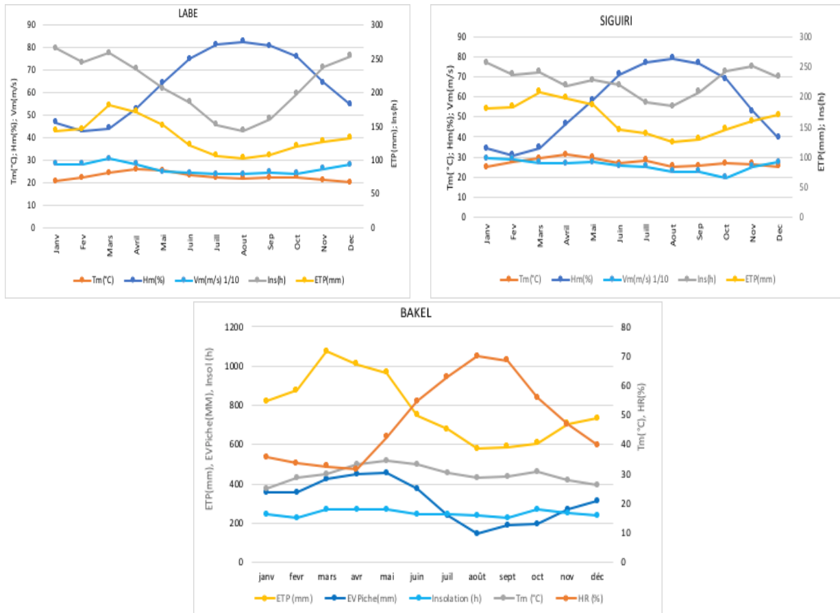
Figure 8: Monthly variation of climatic parameters
