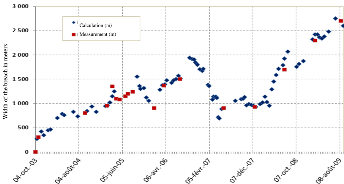
Figure 40: Comparison between the widths of the breach measured in the field and the widths measured from LANDSAT imagery
