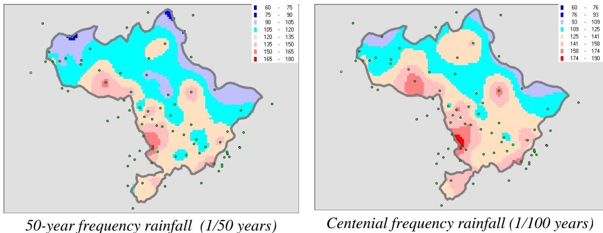
Figure 20 : Spatial distribution map of daily frequency rainfall (mm) over the Senegal basin (Source: Hydrological monograph of the Senegal River, 2011)
