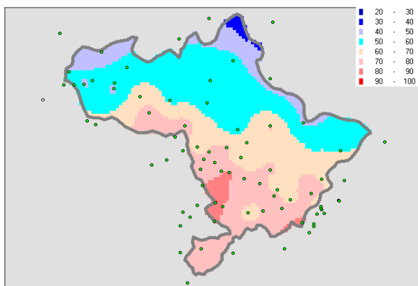
Median frequency rainfall
