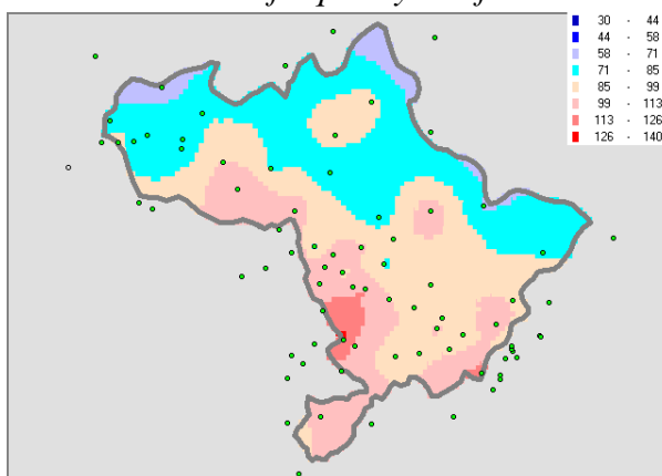
Ten-year frequency rainfall (1/10 years)
