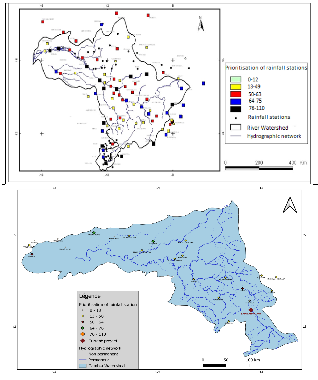
Figure 5: Maps of the rainfall network of the Senegal and Gambia Rivers basins
