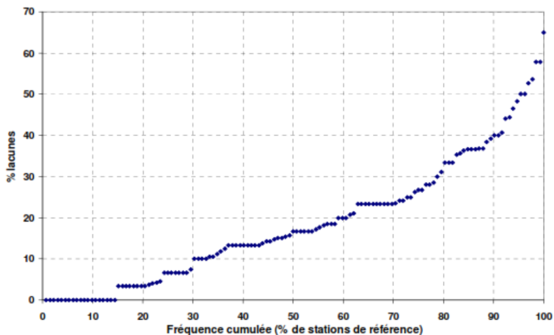
Figure 10: Percentage of gaps in extreme events
