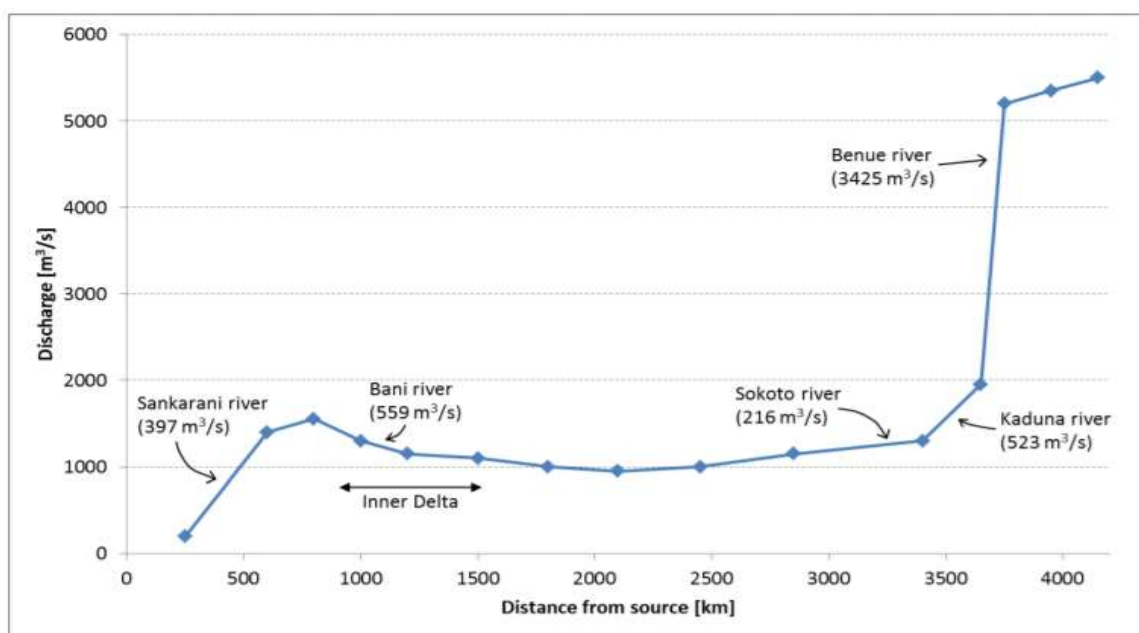
Figure 3.9 Average discharge of the Niger River over its entire length, including the contribution of its main tributaries (adapted from www.fao.org ).
