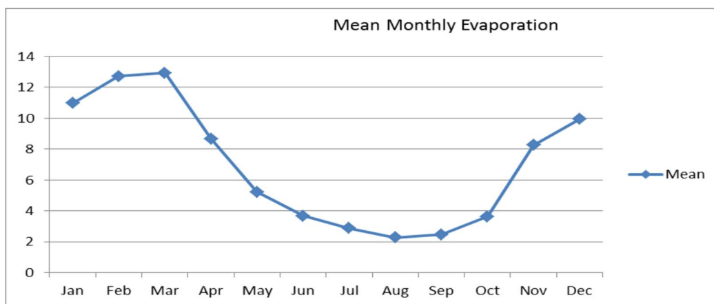
Figure 3.1: Mean Monthly Evaporation in the northern Nigeria (1999 – 2013) in cm
