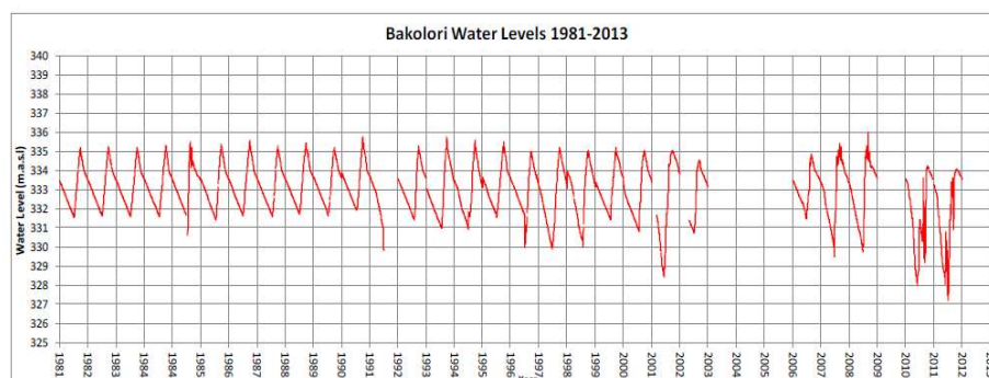
Figure 3.38. Bakolori daily water levels 1981-2013.
