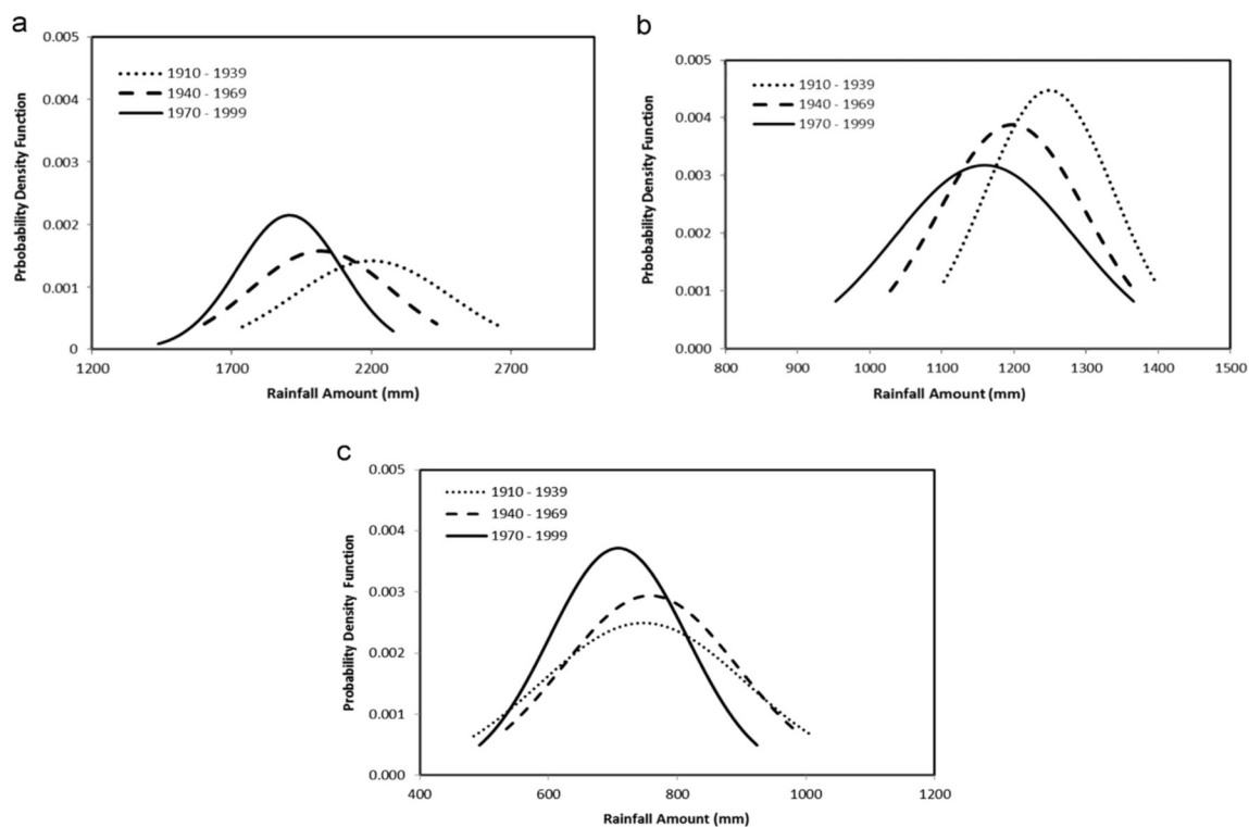
Figure 3.7. Mean annual rainfall distribution over (a) Guinea, (b) Savanna and (c) Sahel.
