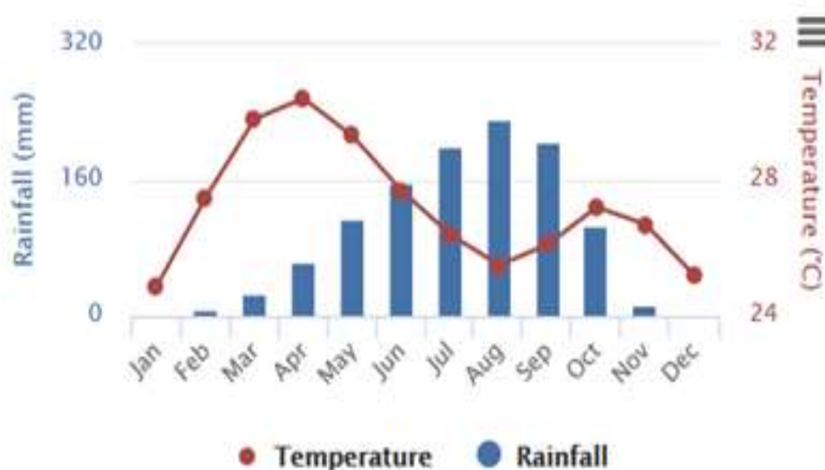
Figure 3.8. Mean monthly temperature and rainfall for Nigeria during 1901-2017.
