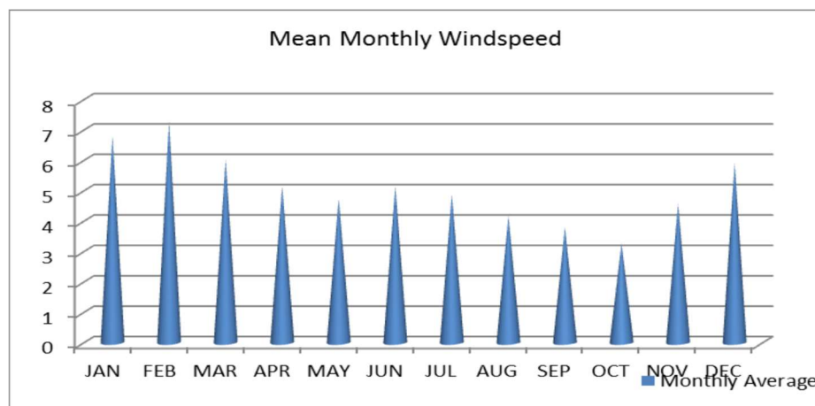
Figure 3.5: Mean Monthly Wind Speed
