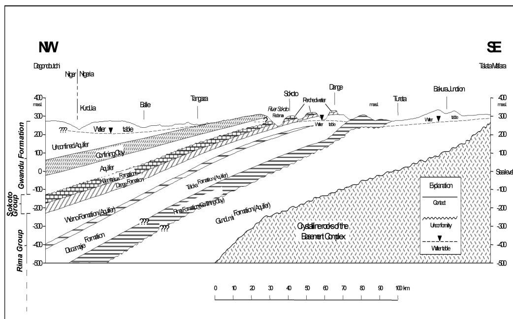
Figure 3.12. Hydrogeological cross-section through Sokoto Basin, North-West Nigeria (modified from Anderson & Ogilbee 1973)
