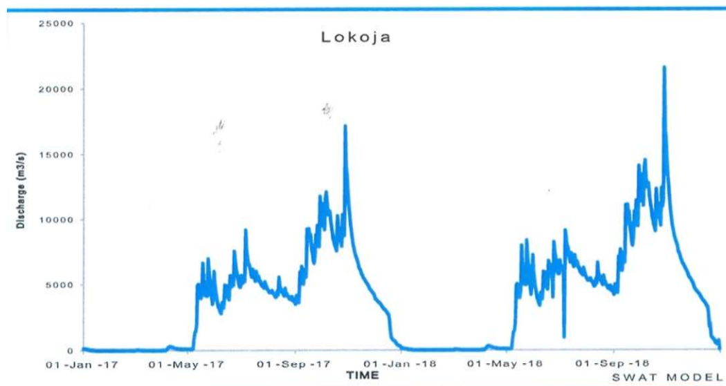
Figure 3.34. Simulation flow at Lokoja, River Niger.
