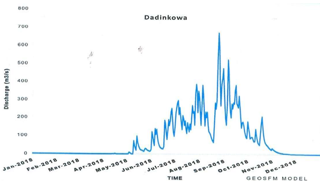
Figure 3.37. Simulation flow at Dadinkowa on Gongola River.
