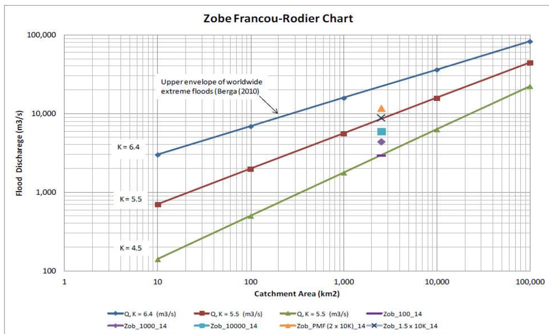
Figure 3.43. Zobe chart design estimates (Francou-Rodier).
