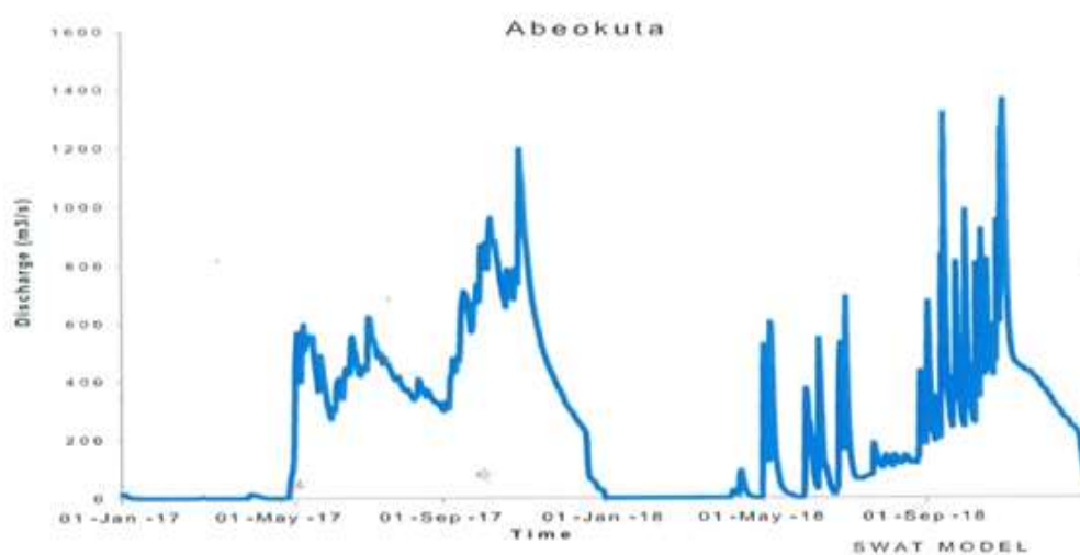
Figure 3.35. Simulation flow at Abeokuta, Ogun River.
