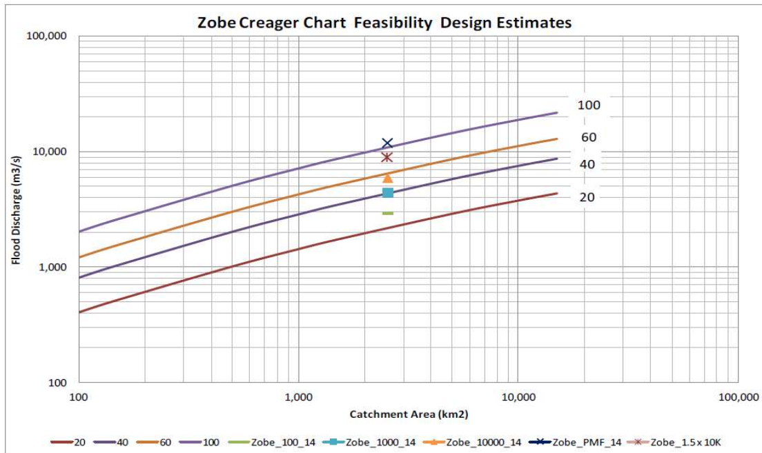
Figure 3.42. Zobe Creager chart design estimates.
