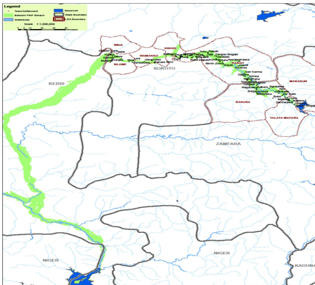
Figure 3.47. Extent of Bakolori breach flood event.
