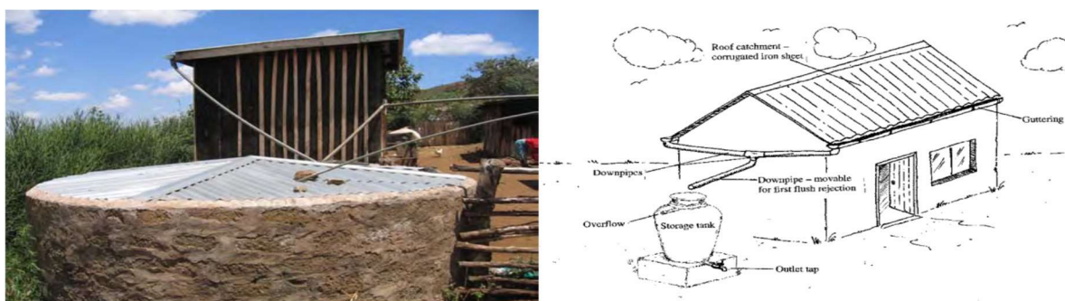
Figure 3.13. Domestic Water Supply: Domestic rain water harvesting
