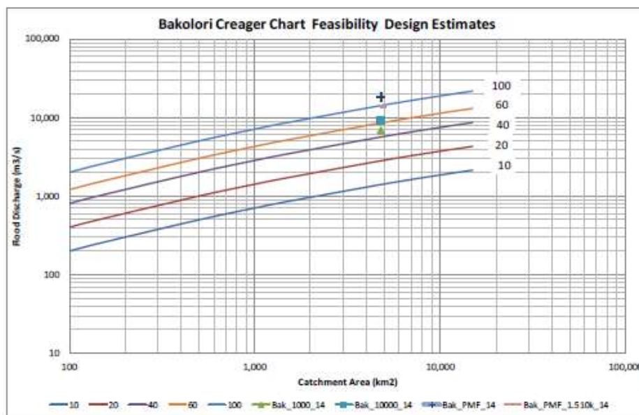
Figure 3.39. Bakolori Creager chart.
