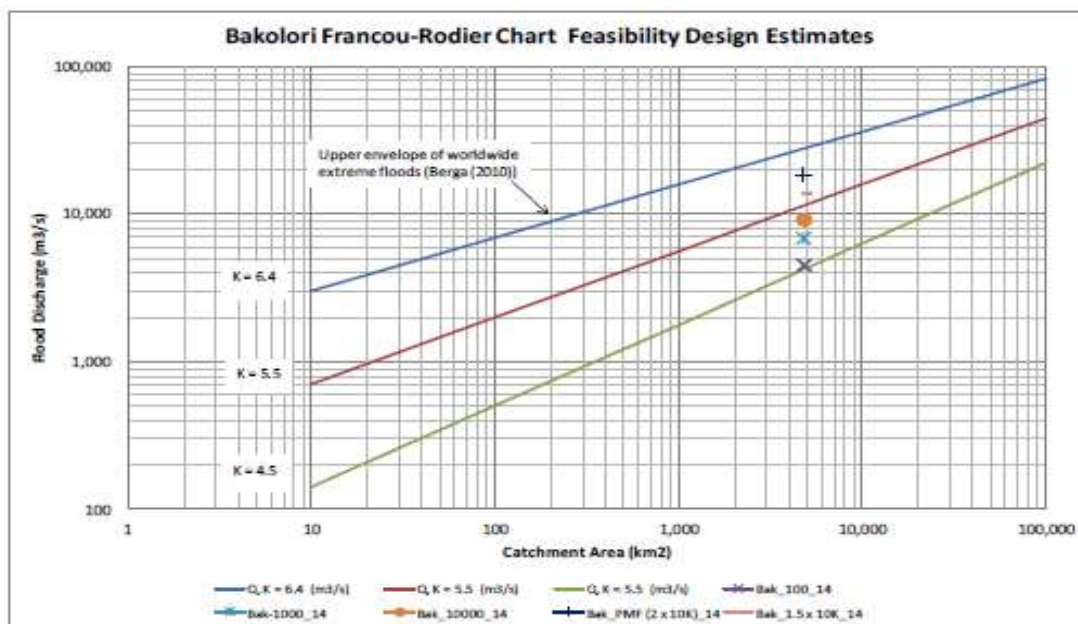
Figure 3.40. Bakolori Francou-Rodier chart.
