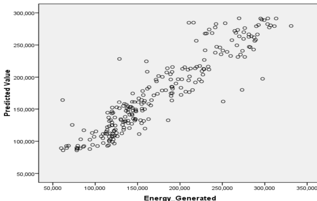
Figure 3.22. Scatter Plot of Predicted and Observed Energy Generated for Jebba HP.
