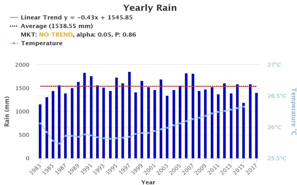
Figure 3.24. Yearly Rain for Niger state (1983 – 2017)
