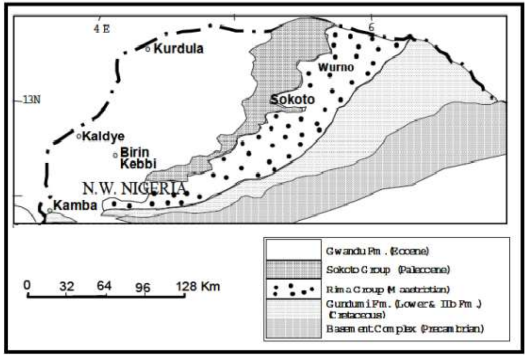
Figure 3.11. Geological map of Nigerian sector of the Iullemedden Basin (after Adelana et al., 2003; modified from Oteze, 1991)
