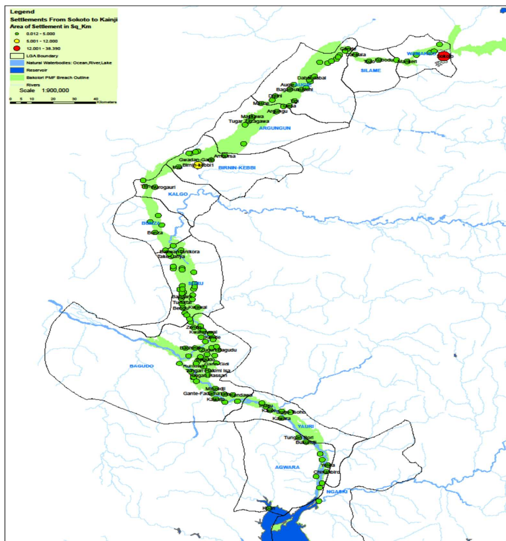
Figure 3.48. Extent of Bakolori breach flood event below Sokoto.
