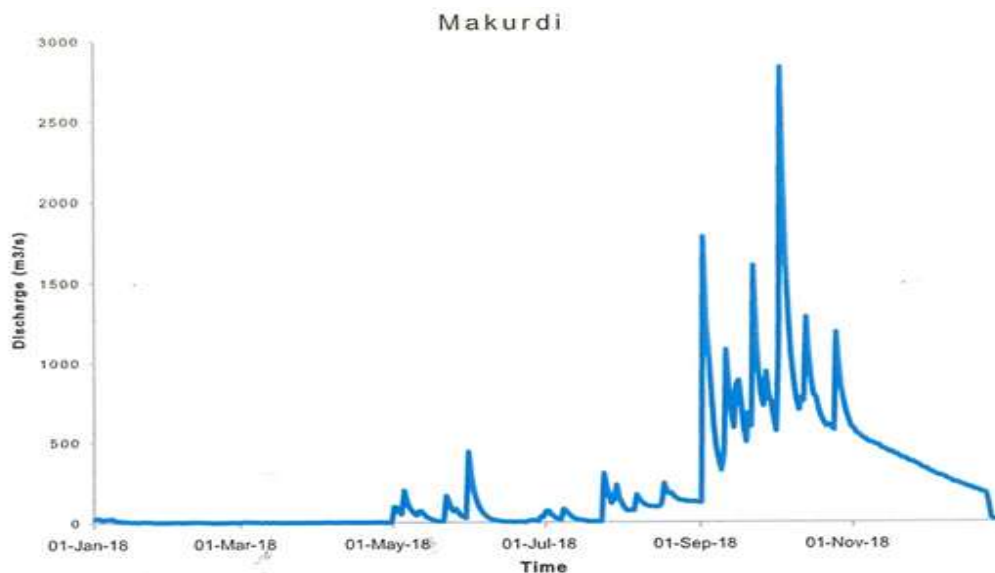
Figure 3.36. Simulation flow at Makurdi, River Benue.
