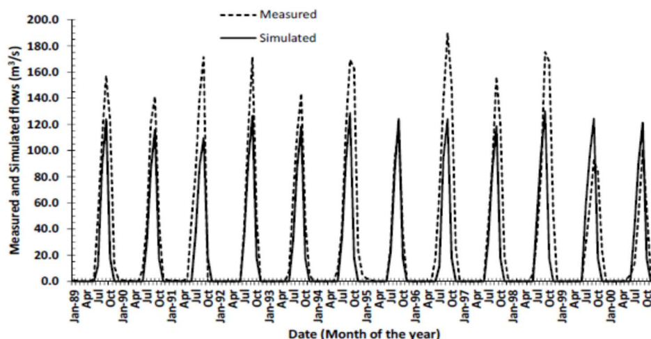
Figure 3.31. Measured average daily flows at Gashua and simulated flows.
