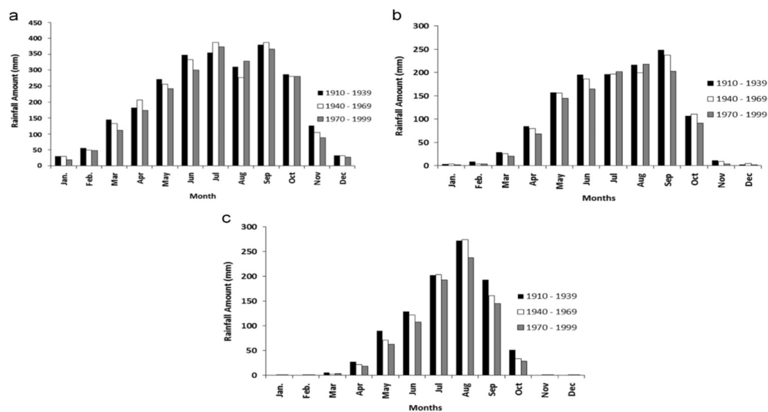
Figure 3.6. Mean monthly rainfall distribution over (a) Guinea, (b) Savanna, and (c) Sahel regions of Nigeria. Source: Stephen and Tobi, 2014
