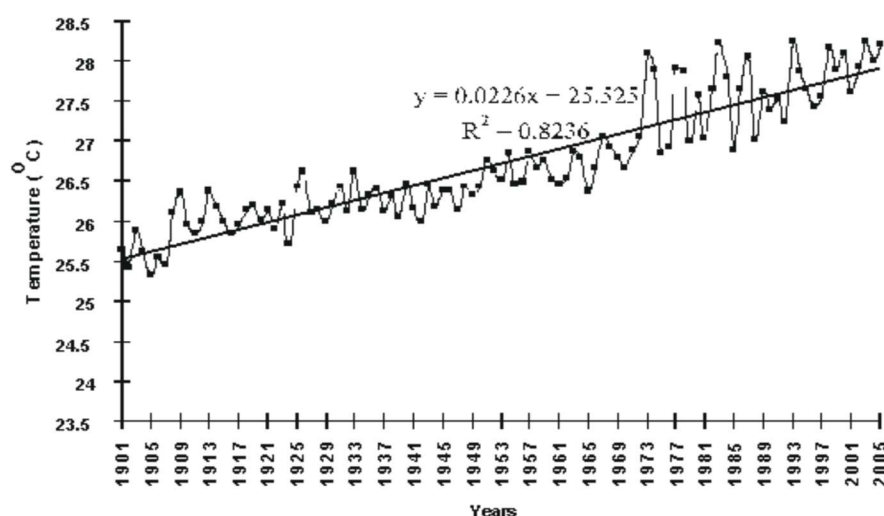
Figure 3.3. Air temperature distribution in Nigeria between 1901 and 2005.
