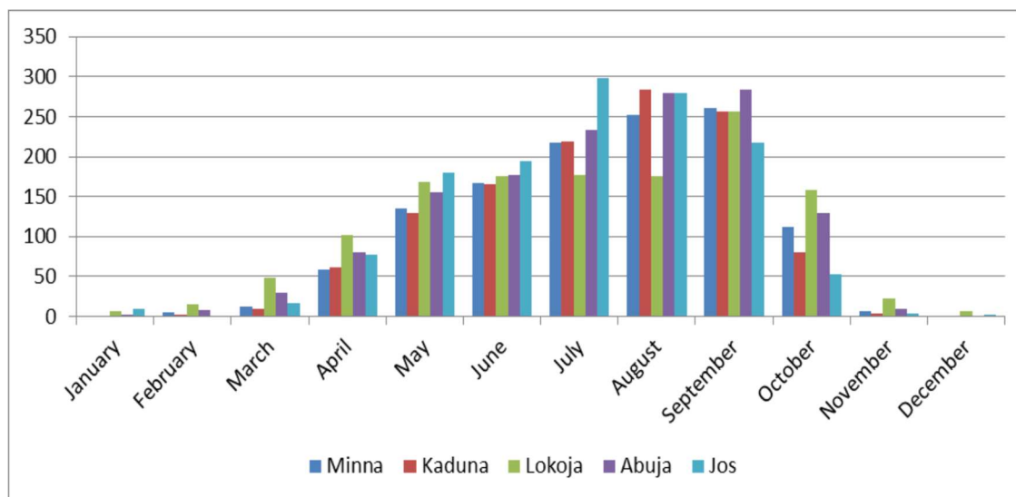
Figure 3.2: Long Term Rainfall at Selected Stations around the northern Nigeria in mm
