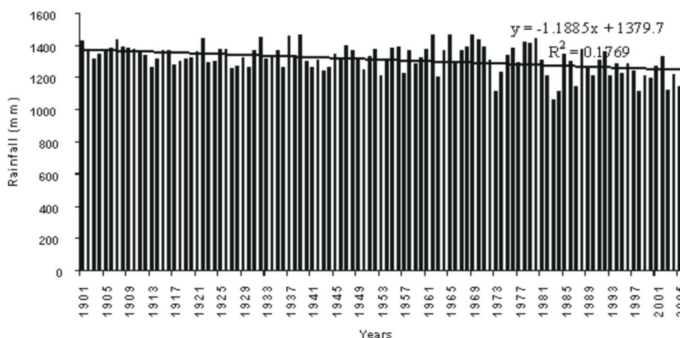
Figure 3.4. Rainfall distribution in Nigeria between 1901 and 2005.
