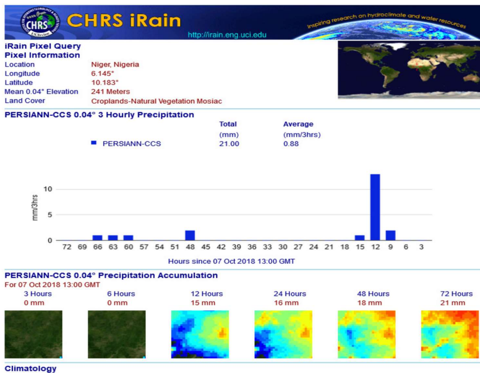
Figure 3.23. 3-hourly Precipitation Accumulation for Niger state.
