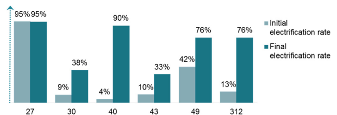
Fig. 15. Impact of PV minigrd implementation on the rate of access to electricity for each settlement.
