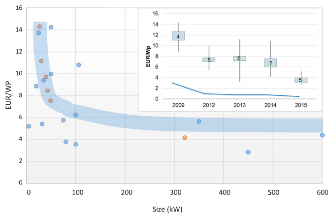
Fig. 7. Full project investment cost variation by PV generator capacity size of the mini-grid (selected samples in red for harmonized study). In box - Full project investment cost variation (number of samples, max and min) by year of procurement. Blue line: corresponding PV module cost for the year of procurement.
